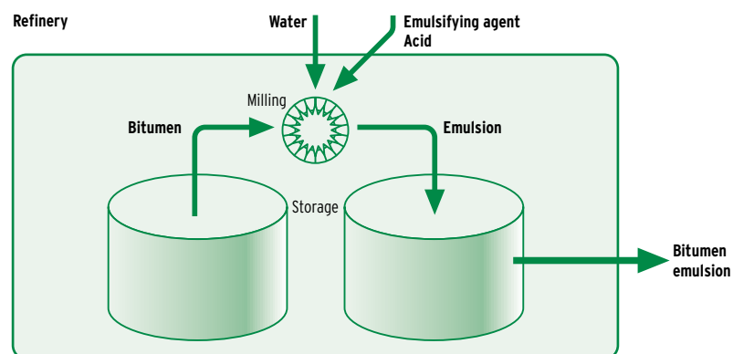
Figure 4. Bitumen emulsion production
