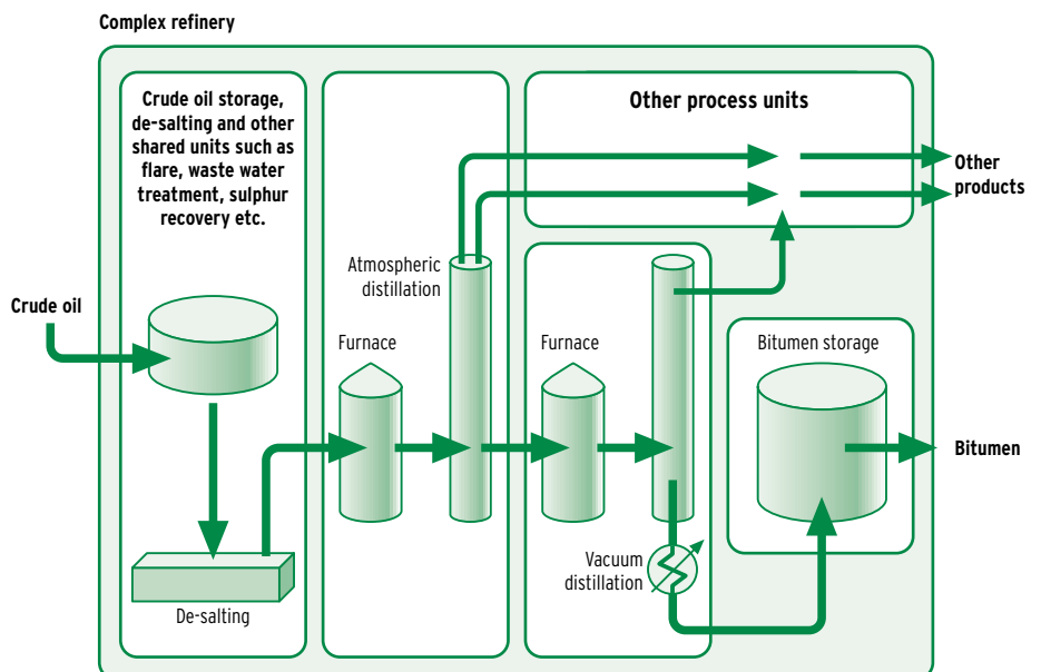
Figure 2. Straight-run distillation of bitumen within a complex refinery
